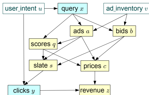
Figure 3: Causal graph associated with the structural equation model of Figure 2. The mutually independent noise variables \varepsilon_1 to \varepsilon_8 are implicit. The variables a , b , q , s , c , and z depend on their direct causes in known ways. In contrast, the variables u and v are exogenous and the variables x and y depend on their direct causes through unknown functions.
